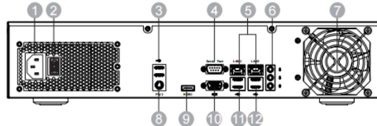
NVR3304 Rear Panel
