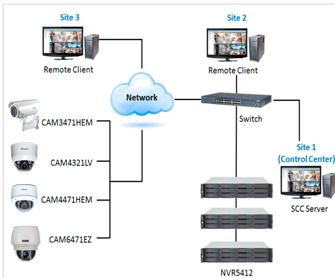
Figure 1: Distributed Architecture
