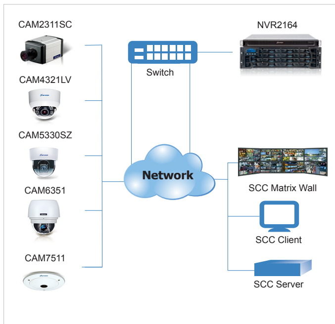
Figure 1: Distributed Architecture for Advanced Applications
