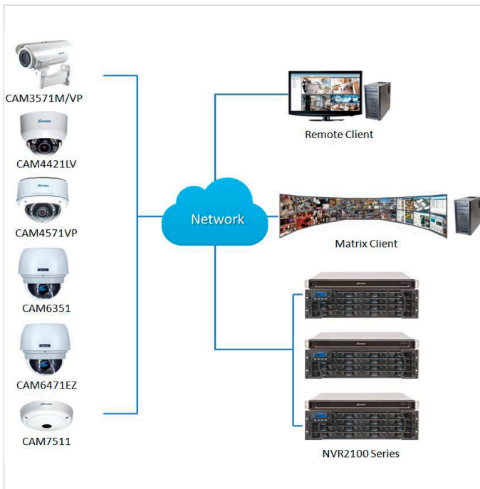
Figure 1: Distributed Architecture
