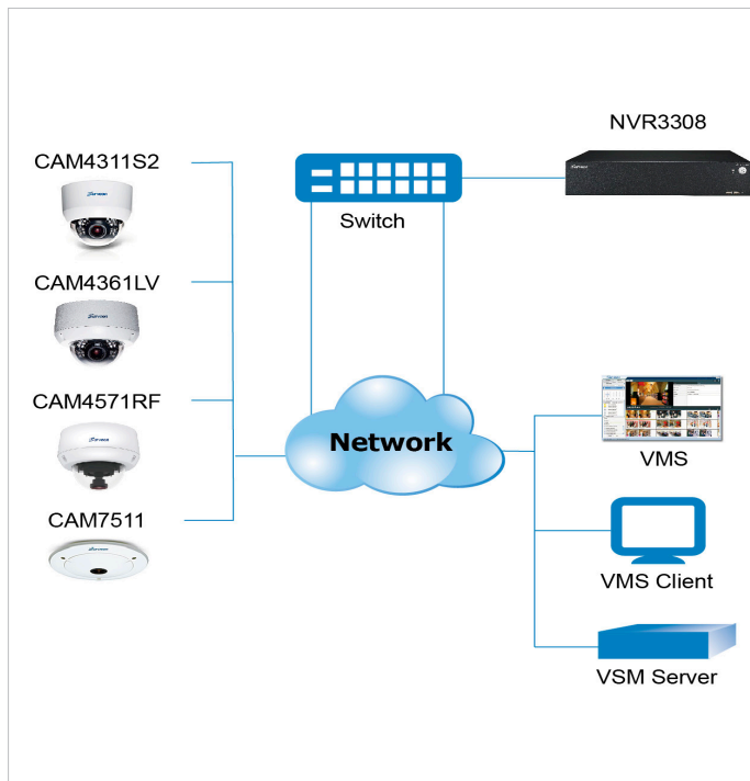
Figure 1: Distributed Architecture
